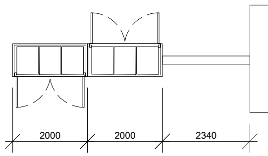
2 Type A Plan 0483
