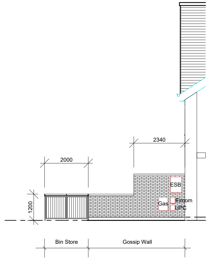
3 Type B Elevation 0483
