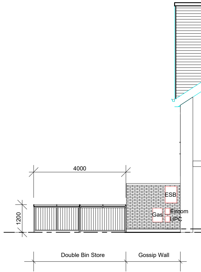
1 Type A Elevation 0483
